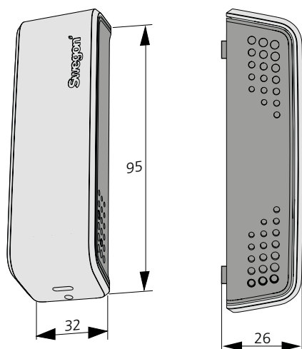
Figure 2. Dimensions, module principal WISE WCS
