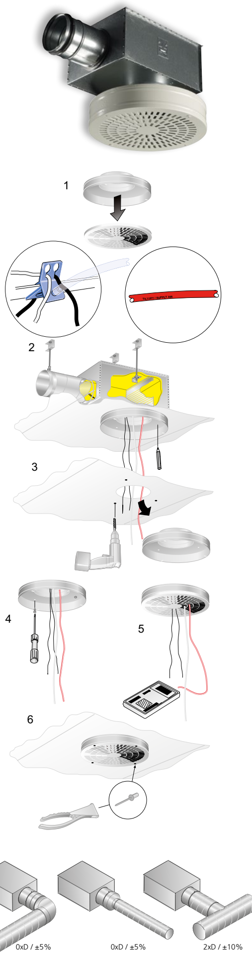
Figure 1. ROC + ALS.
