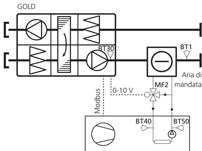
Chiller Swegon
